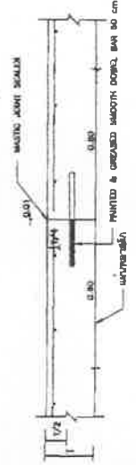
CONSTRUCTION JOINT
