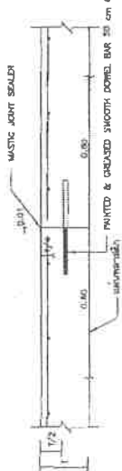
CONSTRUCTION JOINT
