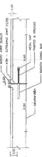
EXPANSION JOINT
