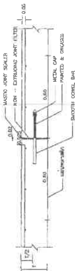
EXPANSION JOINT
